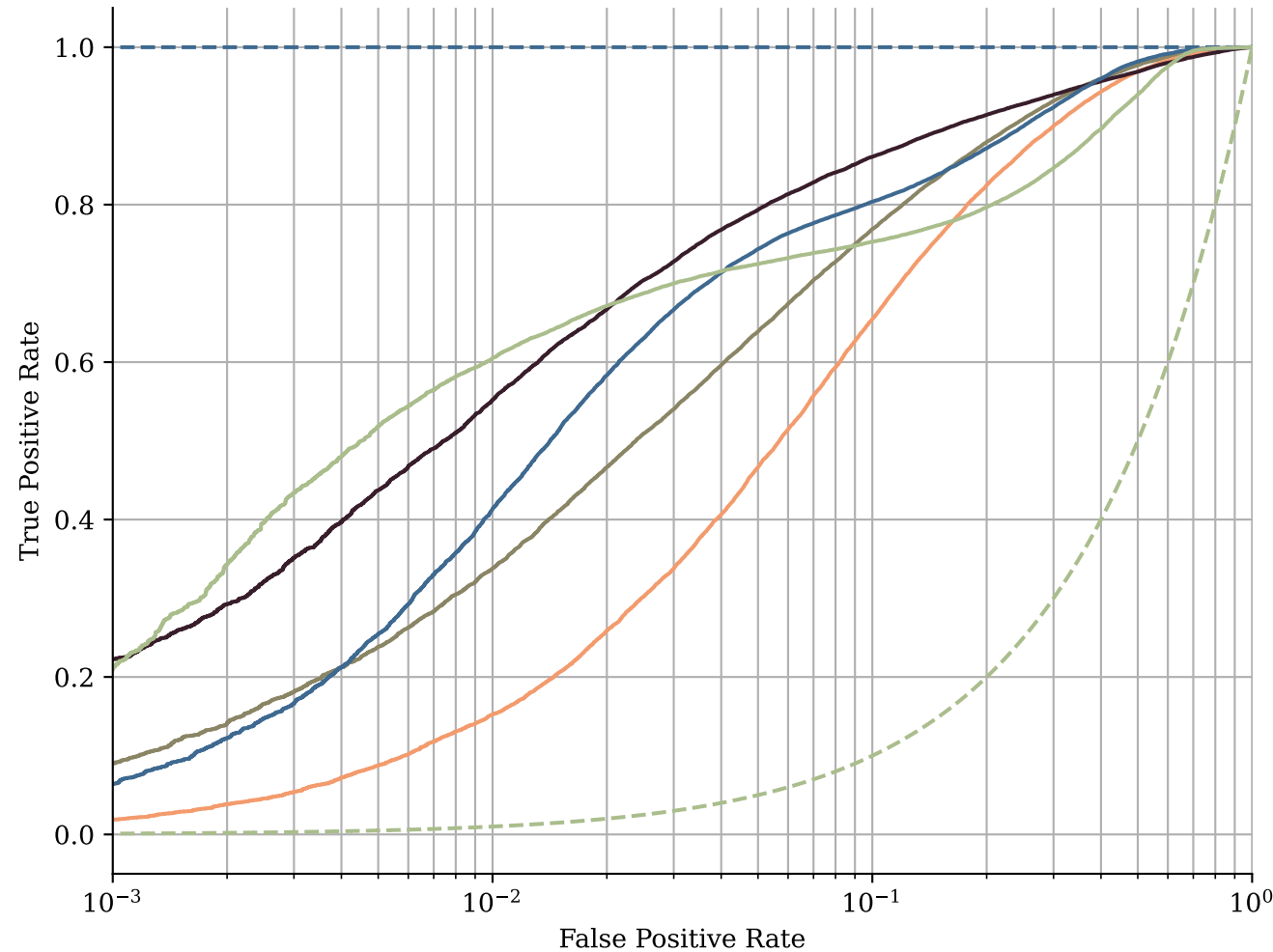
ROC Curves with logarithmic x-axis
